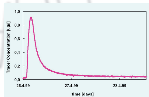
Breakthrough-curve of Eosin in groundwater
